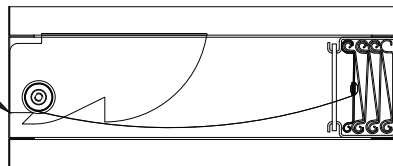
Open Position (38SH or 38DH)
